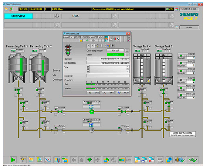
Route Control master module
