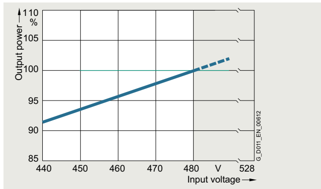
Permissible output power as a function of the input voltage for 400 V SINAMICS G120X converters, frame sizes FSA to FSG, at 100% output current in the range of 440 V to 480 V (the temperature protection of the converter can reduce the current or pulse frequency above 480 V)
