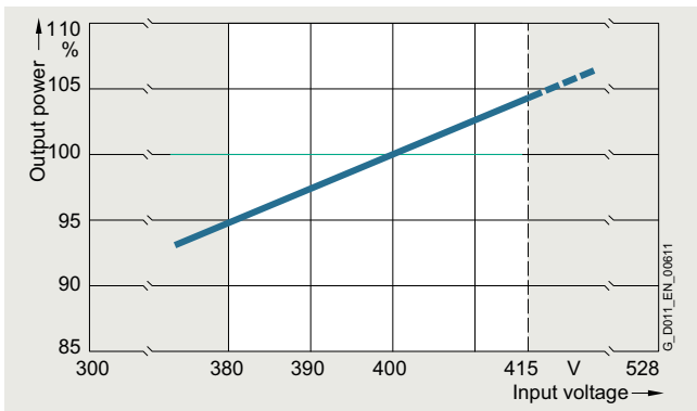
Permissible output power as a function of the input voltage for 400 V SINAMICS G120X converters, frame sizes FSA to FSG, at 100% output current in the range of 380 V to 415 V (the temperature protection of the converter can reduce the current or pulse frequency above 415 V)
