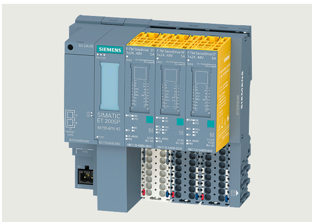
Drive controller modules for ET200SP SIMATIC MICRO-DRIVE F-TM StepDrive ST, ServoDrive HF and ServoDrive ST
