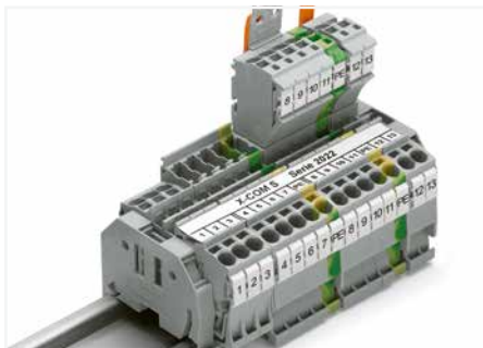
2022 Series X-COM®S-SYSTEM Carrier Terminal Blocks combined with 2002 Series Through Terminal Blocks
