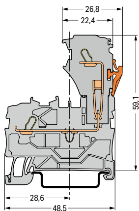
Carrier terminal block
