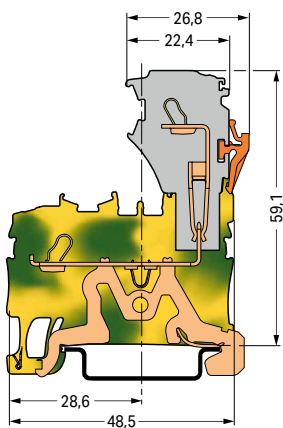
Ground carrier terminal block
