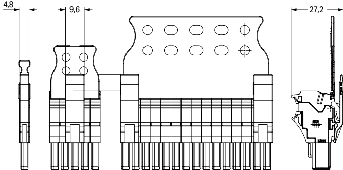
Dimensions of locking levers
