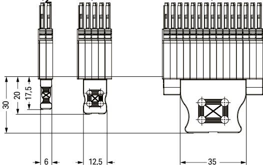
Dimensions of strain relief plates
