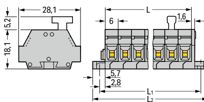
L = pole no. x pole width L 1 = L + 7.2 mm L 2 = L + 13 mm
