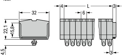
Modular terminal blocks and terminal strips with snap-in mounting feet
