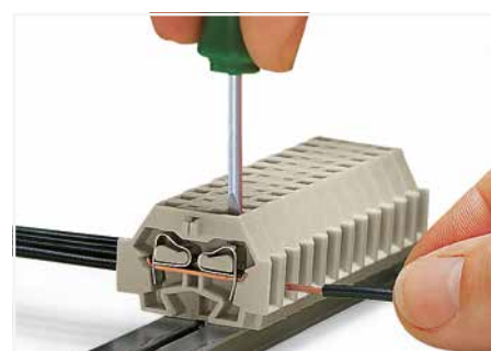
CAGE CLAMP® termination: Inserting a conductor.
