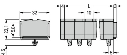
L = (pole no. x pole width) + 7 mm
