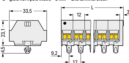
L = (pole no. x pole width) + 3 mm • End terminal block
