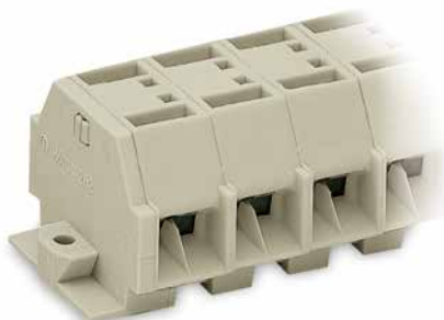
L = pole no. x pole width L 1 = L + 8.1 mm L 2 = L + 14.5 mm
