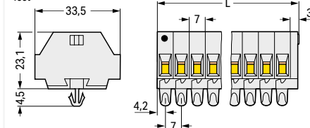
Modular terminal blocks and terminal strips with snap-in mounting feet
