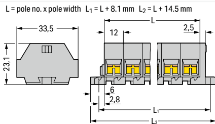
Terminal strip; with mounting flanges; for screw or similar mounting types; 3.2 mm mounting hole diameter (with 209-123 Mounting Foot for DIN-35 rail)
