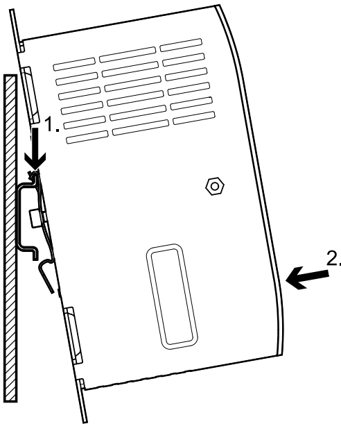
Fig. 10 Mounting on an H-rail
