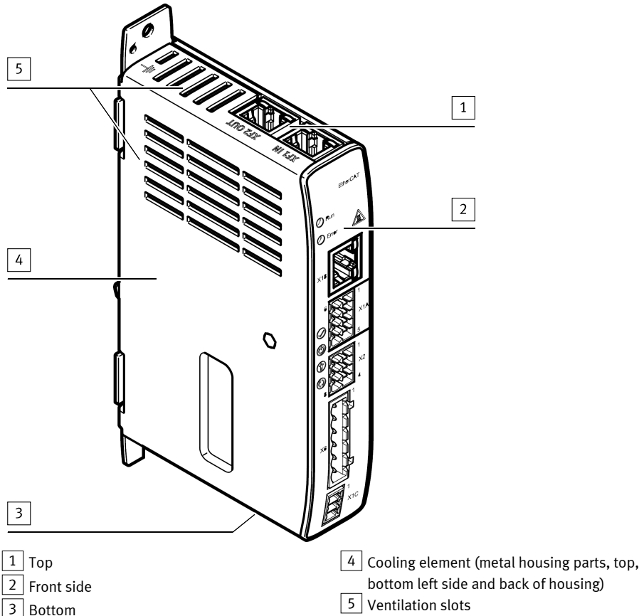
Fig. 4 Servo drive CMMT-ST
