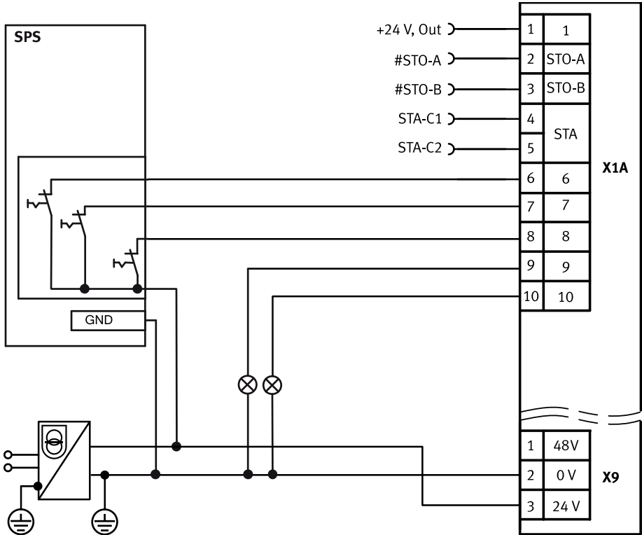
Fig. 12 Connection example, PNP logic
