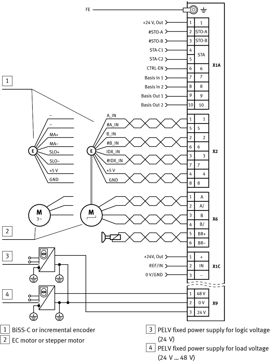
Fig. 11 Connection example
