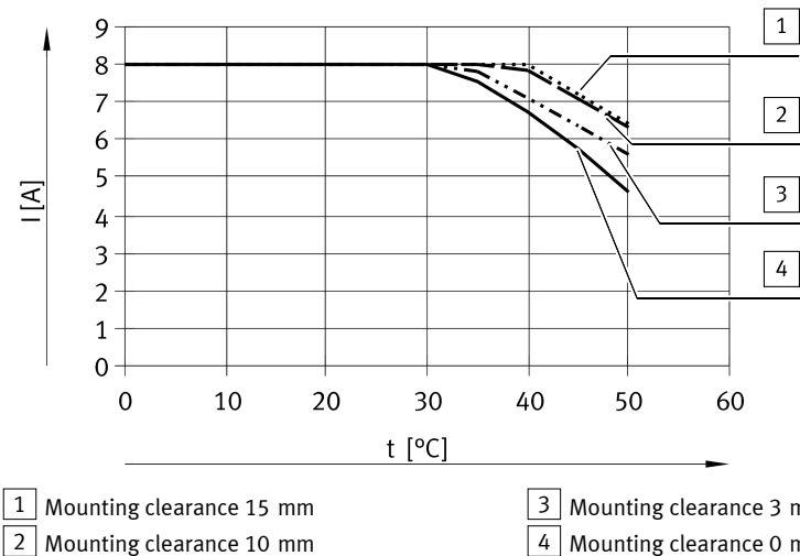
Fig. 16 Power reduction as a function of the ambient temperature and mounting clearance
