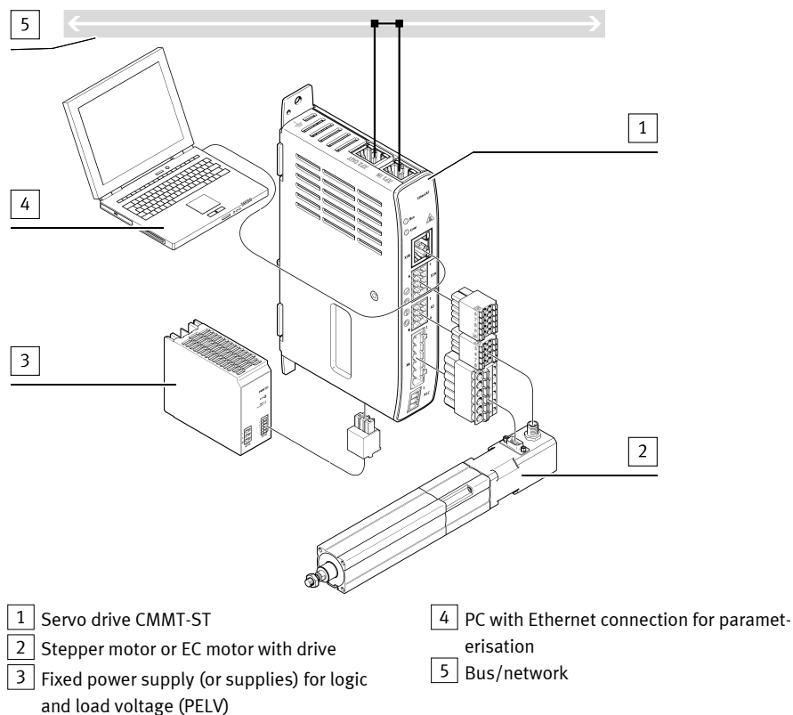
Fig. 3 System structure (example)
